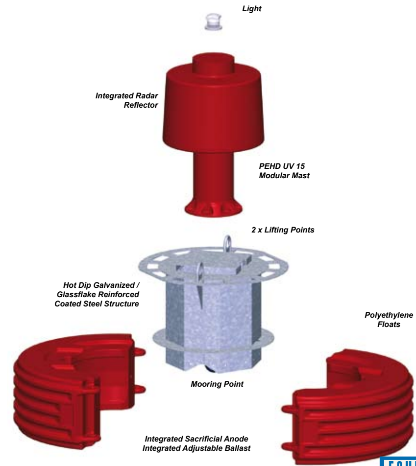
Exploded view of a JET 1400
