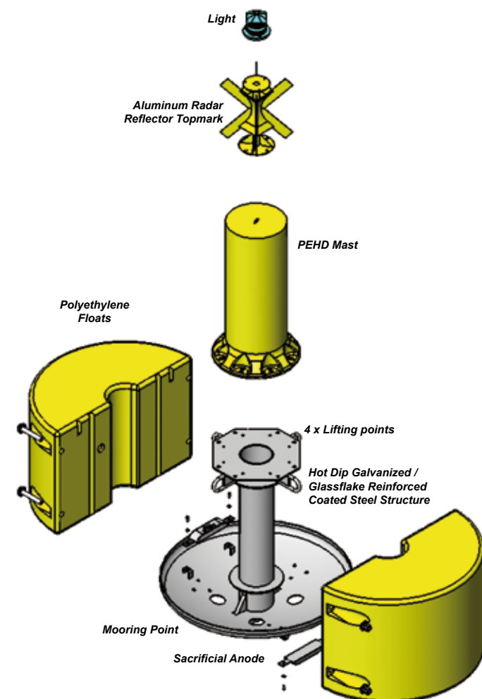
Exploded view of a FB 1242
