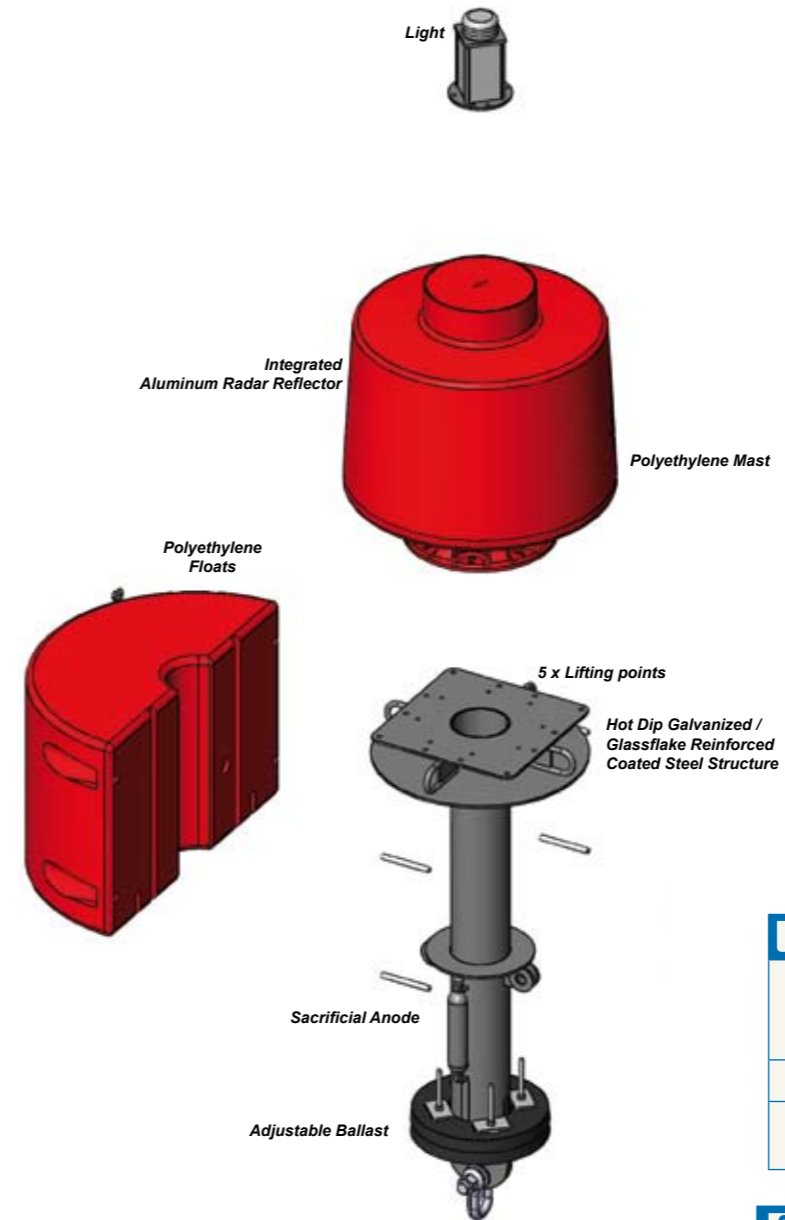
Exploded view of a BC 1242
