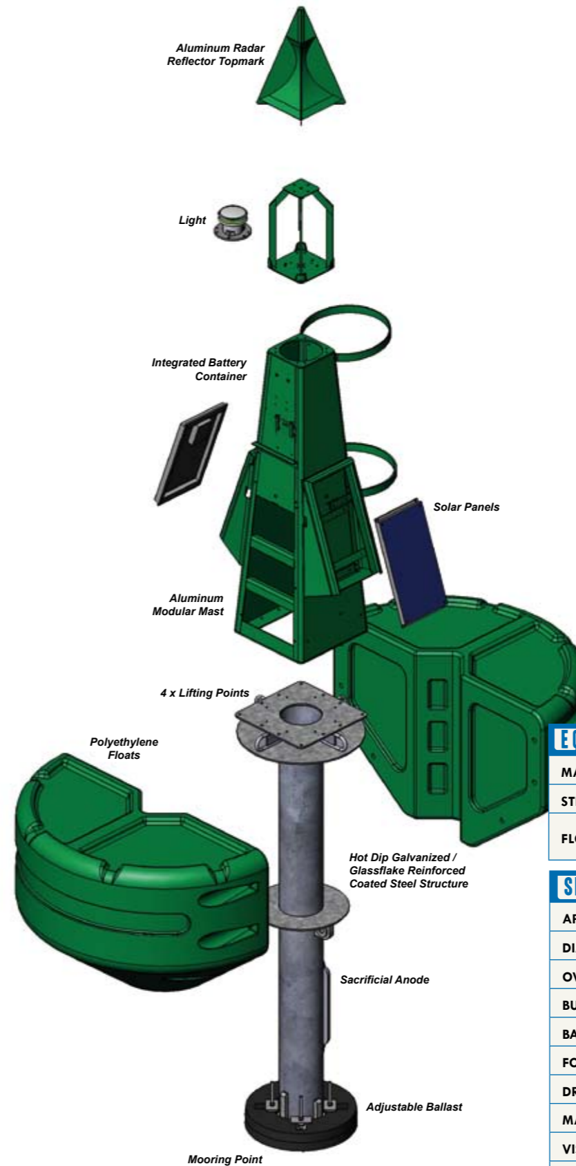
Exploded view of a JET 2500 Q PF3
